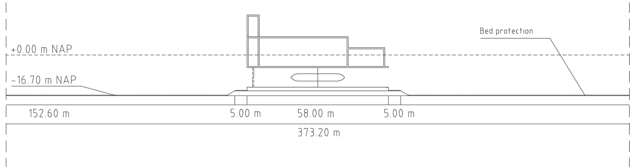
Figure 52. Tidal power plant cross-section with bed protection length
