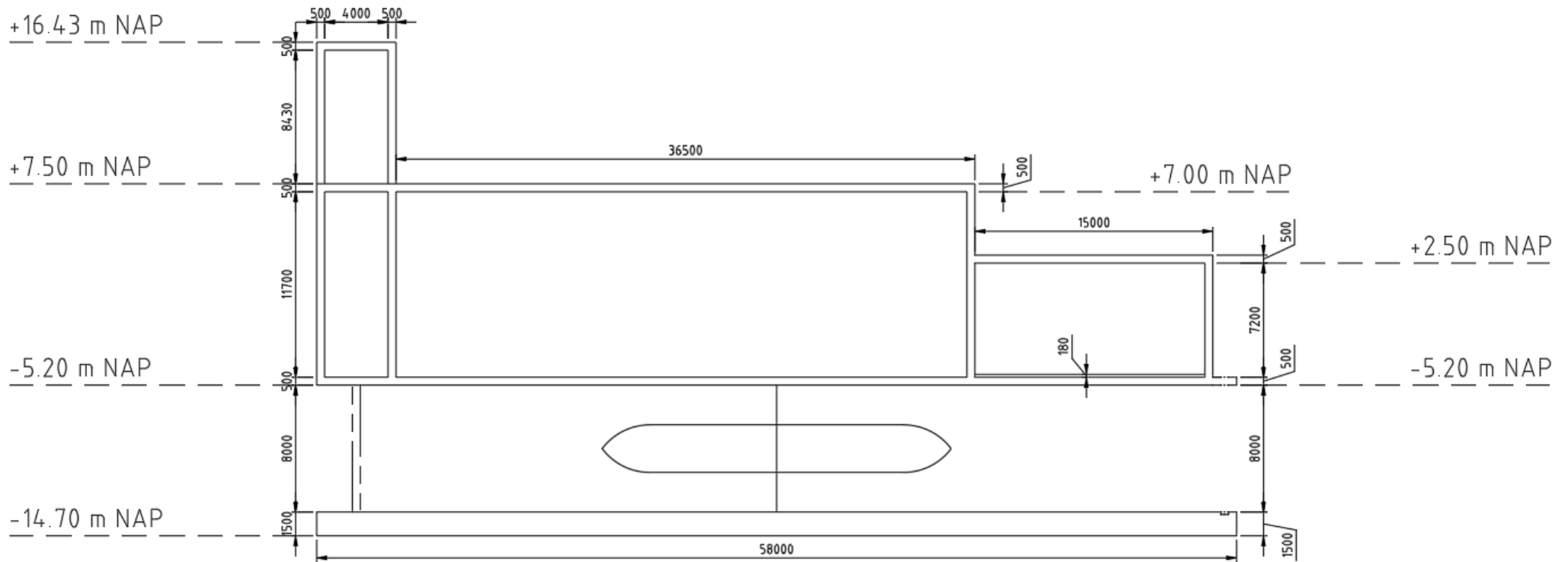
Figure 48. Transversal cross section of the tidal power plant
